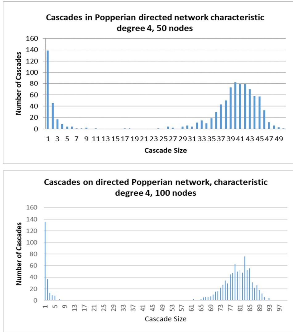
Fig. 17 Comparative cascade sizes in Popperian networks of 50 and 100 nodes
