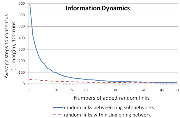
Fig. 4. The importance of degree of linkage in time to belief consensus: Contrast between results of adding additional linkages within a single ring network (below) and between ring sub-networks (above)
